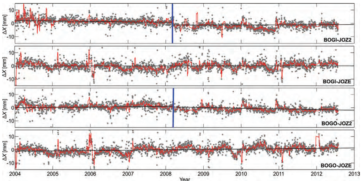
Fig. 2. Variations in X-component; daily solutions (grey dots) and 7-day average solutions (red line); linear trends (black line); blue vertical lines represent the period of antenna replacement at JOZ2
