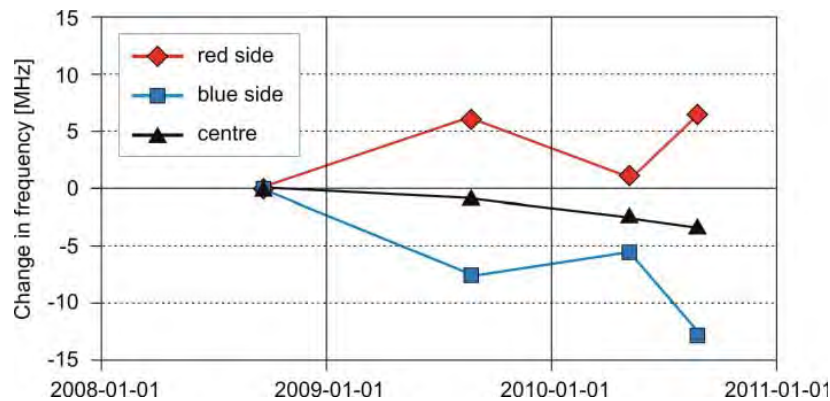
Fig. 9. The calibrations of the laser of the A10-020 for the two side locks and the centre frequency. The change in frequency is shown relative to the first calibration at Micro-g LaCoste, Inc. Subsequent calibrations were performed at MIKES. Uncertainties are not shown. A change of 1 MHz in the laser frequency corresponds to 2.1 \mu\text{Gal} in measured gravity. The total drift of the centre frequency in two years was 3.1 MHz which, if neglected in the processing, would lead to an error of 6.4 \mu\text{Gal} in measured gravity
