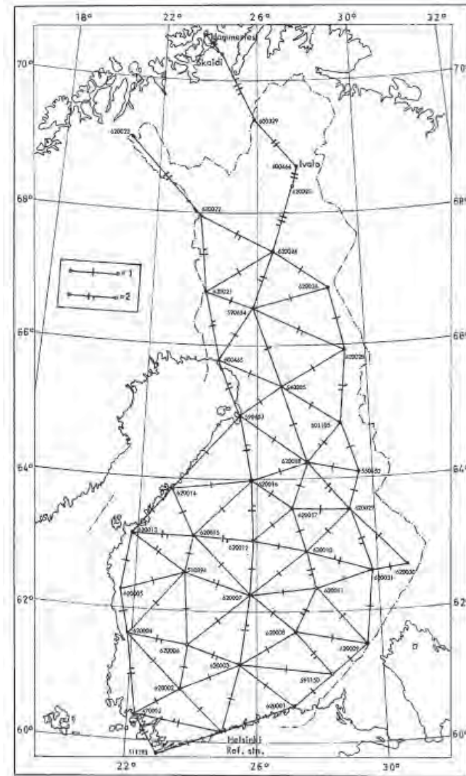
Fig. 3. The First Order Gravity Network of Finland measured in 1962–63 (Kiviniemi, 1964). The tags on the connecting lines indicate the number of measurements of the gravity difference. One cross-tag: measurement of the type ABA; one and a half cross-tags: measurement ABAB, etc.
