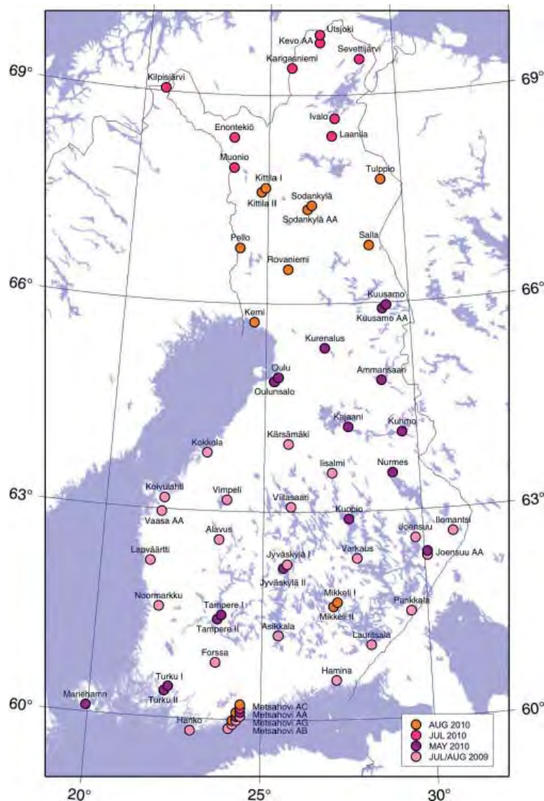
Fig. 7. Stations occupied with the A10-020 in 2009 and 2010. The FOGN network is slightly expanded and densified compared with the original in Figure 3. Some towns have more than one FOGN station; the roman numbers used here to distinguish the sites are not the official FOGN names. The laboratory-type absolute-gravity sites where comparisons with measurements by the FG5-221 were made have two letters after the name
