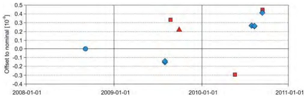
Fig. 8. The relative offset of the frequency of the rubidium oscillator of the A10-020. The nominal frequency of the oscillator is f = 10 MHz. The plotted number is \Delta f/f where f + \Delta f is the measured frequency. The blue circle is the initial calibration at Micro-g LaCoste, Inc. The blue diamonds are our own calibrations at the Metsähovi Geodetic Observatory. The red triangle corresponds to the calibration at BIPM. The red squares show the results of the calibrations at MIKES. Uncertainties are not plotted
