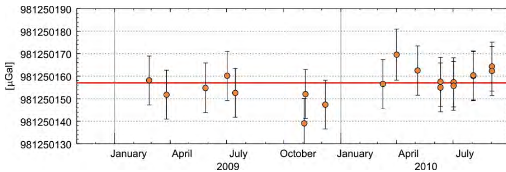
Fig. 2. Results of measurements with the A10-020 at the field station 156 Borowa Gora. The red line corresponds to the average of all measurements with the A10-020
