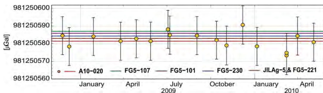
Fig. 1. Results of measurements with the A10-020 at the A-BG laboratory station in the Borowa Gora Observatory. The error bars are provided by the default settings in the “g8” acquisition and post-processing software provided by Micro-g LaCoste, Inc. The 10 \mu\text{Gal} uncertainty from “System Type” is always the dominant contribution. The red line corresponds to the average of all measurements with the A10-020
