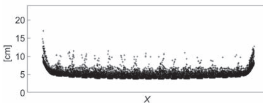
Figure 7. Block A, GCPs distribution variant No. 3, average level of measurement precision. Precision distribution of X coordinate of object points. 3D view of 20 091 standard deviation of object points. View into the depths of 110 photos
